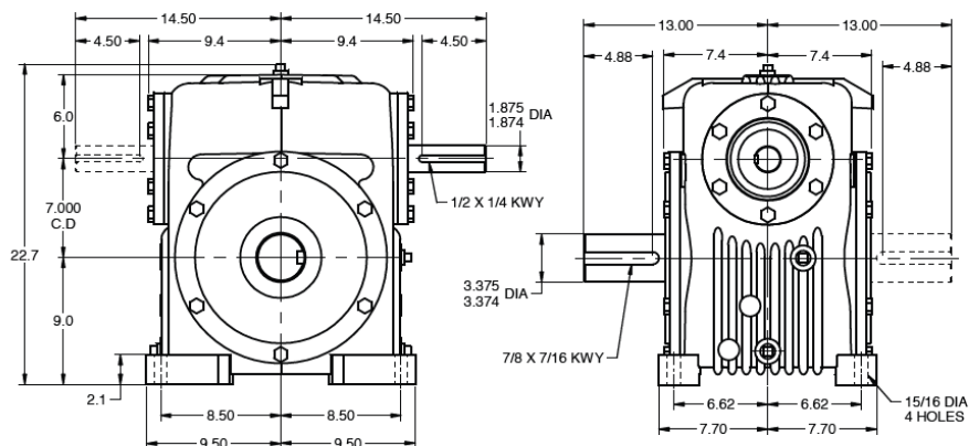
Model HvD070 – Worm Under Gear net wt. 605 lbs
