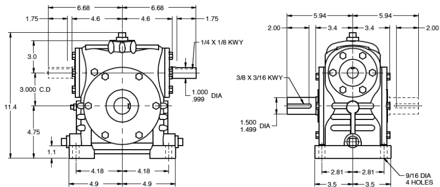
Model HvD030 – Worm Over Gear net wt. 73 lbs
