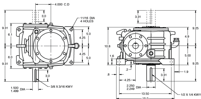
Model HvD040 – Vertical Gear Shaft
