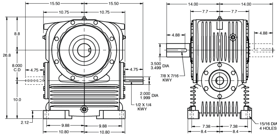
Model HvD080 – Vertical Gear Shaft
