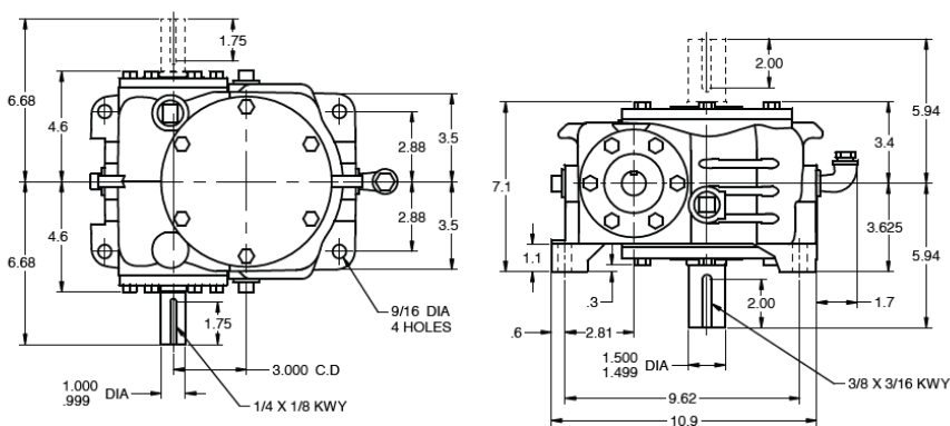
Model HvD030 – Vertical Gear Shaft
