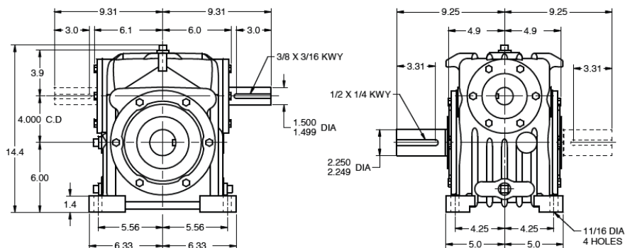
Model HvD040 – Worm Over Gear net wt. 175 lbs
