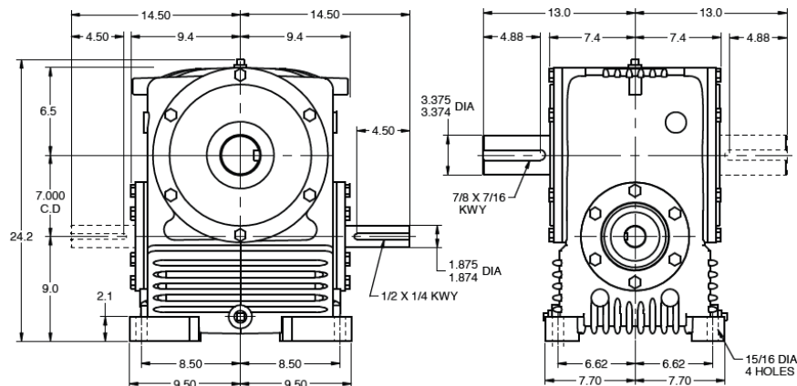
Model HvD070 – Vertical Gear Shaft
