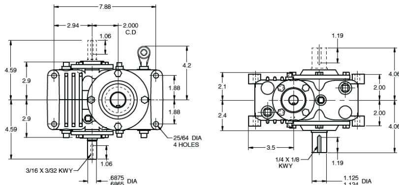
Model HvD020 – Vertical Gear Shaft
