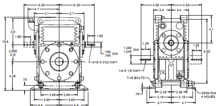
Model HvD025 – Worm Under Gear net wt. 45 lbs
