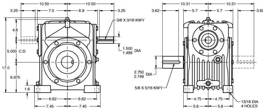
Model HvD050 – Worm Under Gear net wt. 305 lbs
