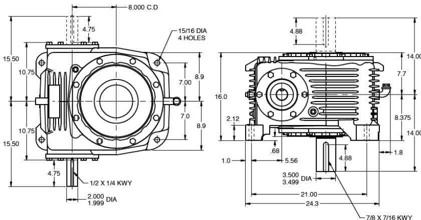
Model HvD080 – Vertical Gear Shaft
