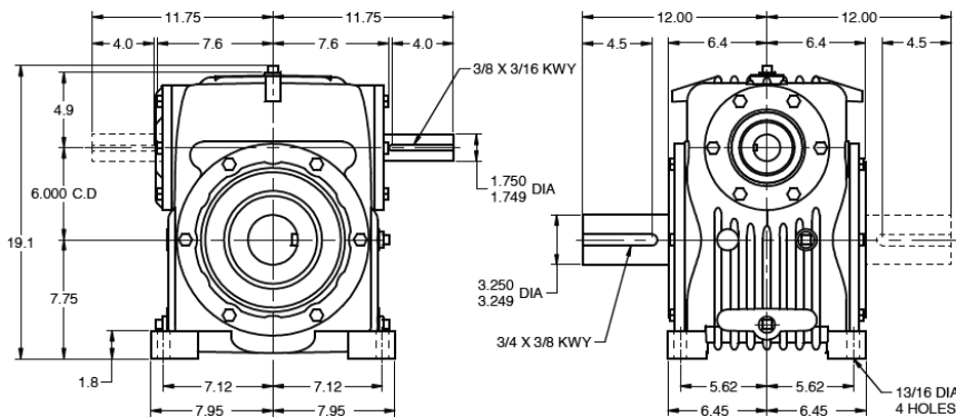
Model HvD060 – Worm Under Gear net wt. 396 lbs
