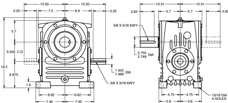
Model HvD050 – Vertical Gear Shaft
