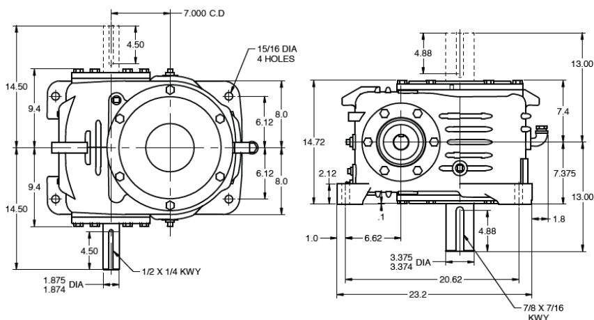
Model HvD070 – Vertical Gear Shaft
