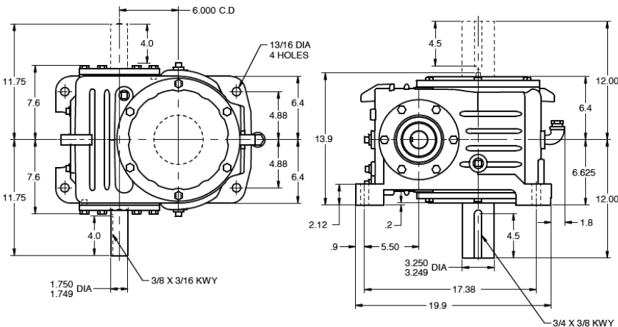
Model HvD060 – Vertical Gear Shaft
