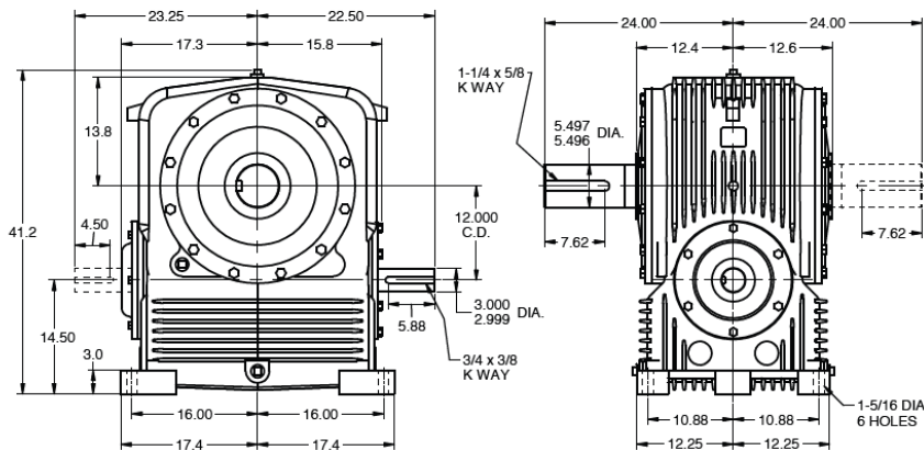
Model HvD120 – Worm Under Gear net wt. 2775 lbs.
