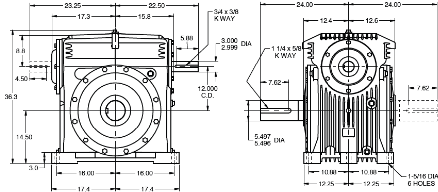
Model HvD120 – Worm Under Gear net wt. 2775 lbs.
