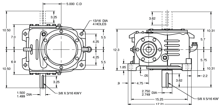
Model HvD050 – Vertical Gear Shaft
