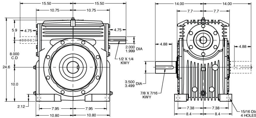
Model HvD080 – Worm Under Gear net wt. 880 lbs
