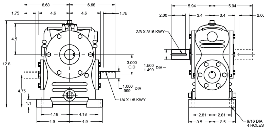
Model HvD030 – Vertical Gear Shaft
