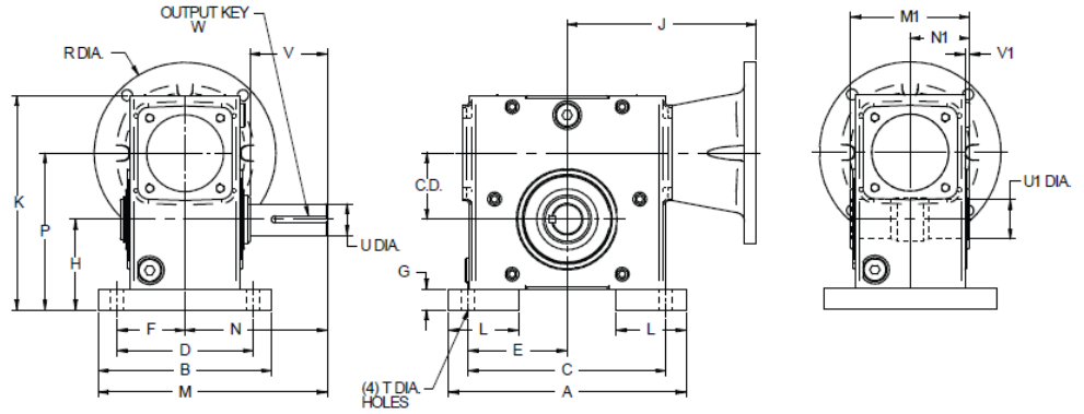
MOTORIZED
