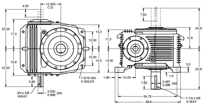
Model HvD120 – Vertical Gear Shaft
