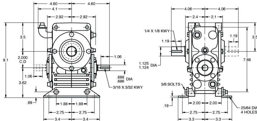
Model HvD020 – Worm Under Gear net wt. 26 lbs
