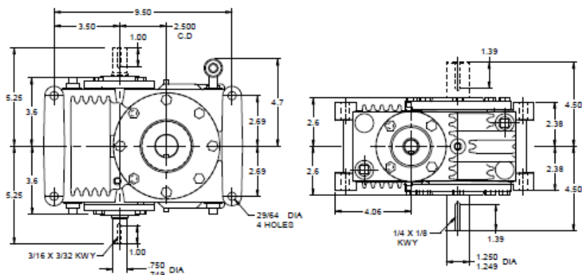
Model HvD025 – Vertical Gear Shaft
