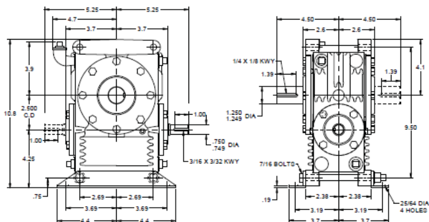
Model HvD025 – Worm Under Gear net wt. 45 lbs
