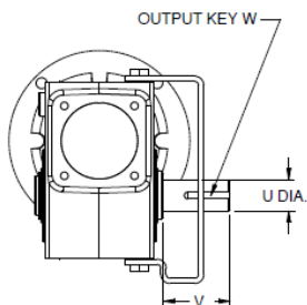
MOTORIZED
