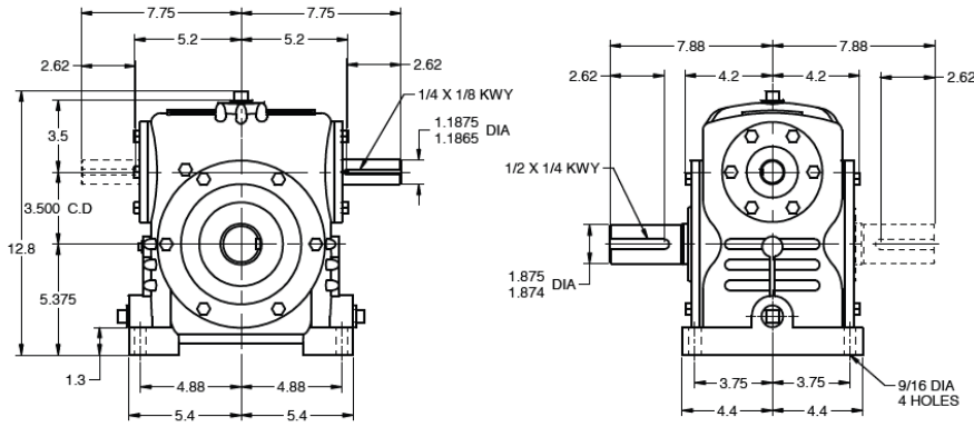
Model HvD035 – Worm Over Gear net wt. 122 lbs
