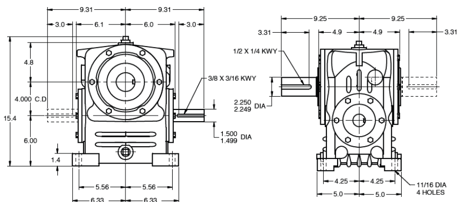
Model HvD040 – Worm Under Gear net wt. 187 lbs
